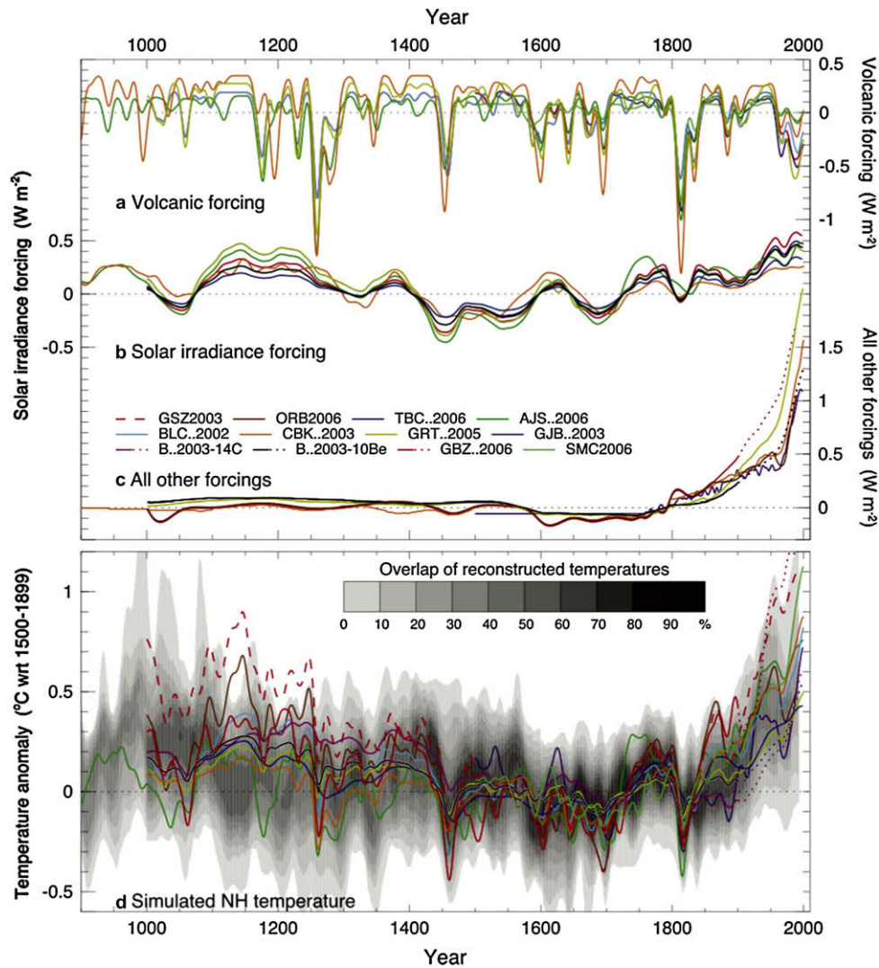
Fig. 16. Radiative forcings and simulated temperatures during the last 1.1 kyr. Radiative forcing ( W/m^2 ) used to drive climate model simulations due to (a) volcanic activity, (b) solar irradiance variations and (c) all other forcings. (d) Annual mean NH temperature ( ^{\circ}C ) simulated under the range of forcings shown in (a) to (c), compared with the concentration of overlapping NH temperature reconstructions (shown by grey shading). All forcings and temperatures are expressed as anomalies from their 1500 to 1899 means and smoothed with a Gaussian-weighted filter. From Jansen et al. (2007).
